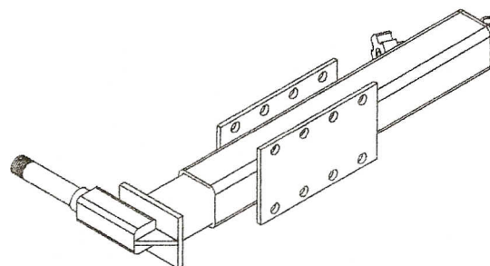
GAUGE WHEEL
